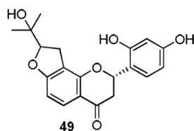
Fig. (4). Structures of natural product flavanones tested for aromatase inhibition.
