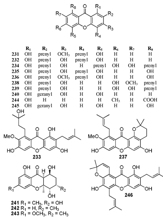
Fig. (16). Structures of natural product xanthenes tested for aromatase inhibition.
